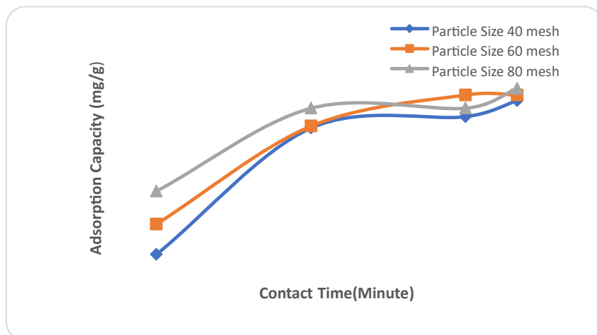
Fig 1. Graph of Relationship Between Contact Time and Adsorption Capacity
