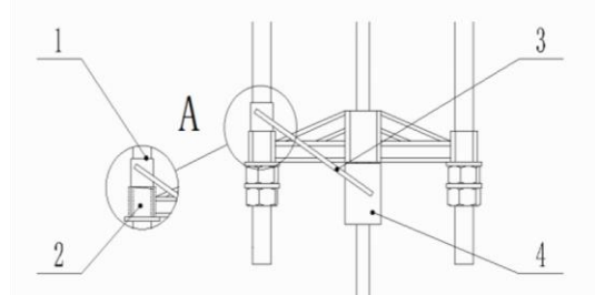
1-Bevelled round tube (bottom) 2-Bevelled round tube (top) 3-Connecting rod 4-Limiting block
