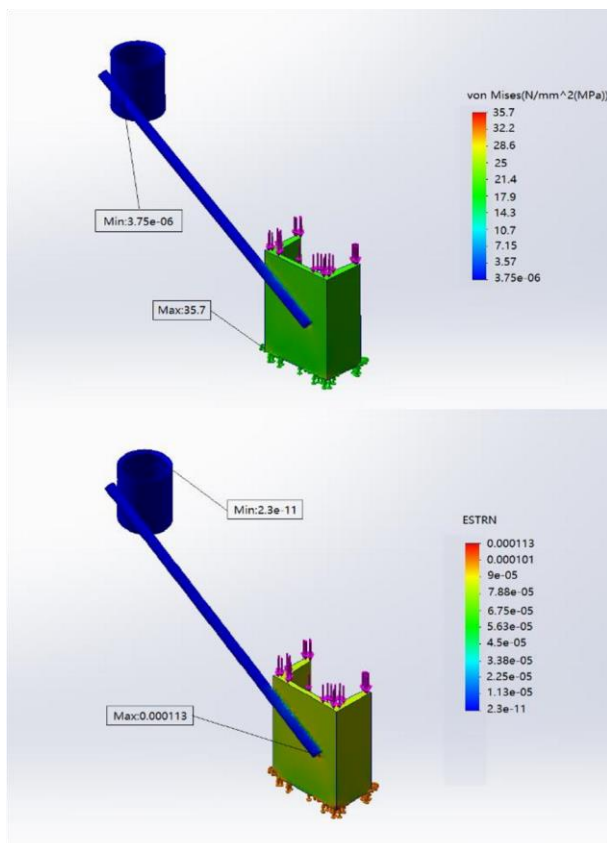
Figure 10: Stress-strain cloud diagram of limit device
