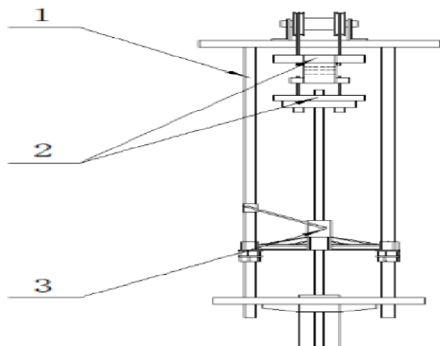
1 - Wellhead support 2 - Overload protection module 3 - Auxiliary unloading module Figure 1: General assembly sketch of wellhead unloading protection device
