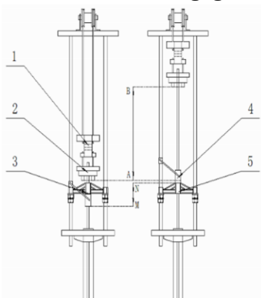
Figure 2: Schematic diagram of the working principle of LPS suspension rope assisted unloading device
