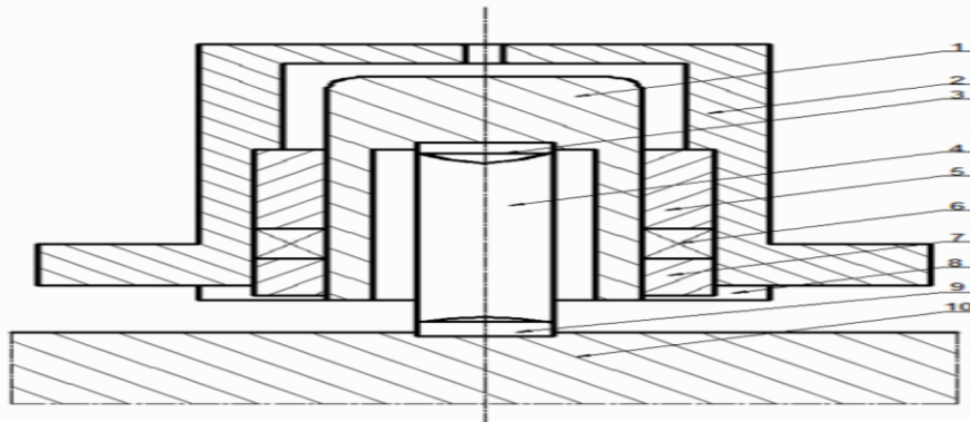
Figure 1: Structure of the cylinder.
