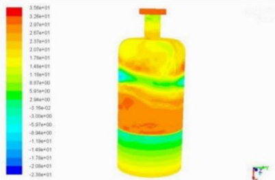
Figure 10: Fluid pressure distribution in the fluid–structure interaction
