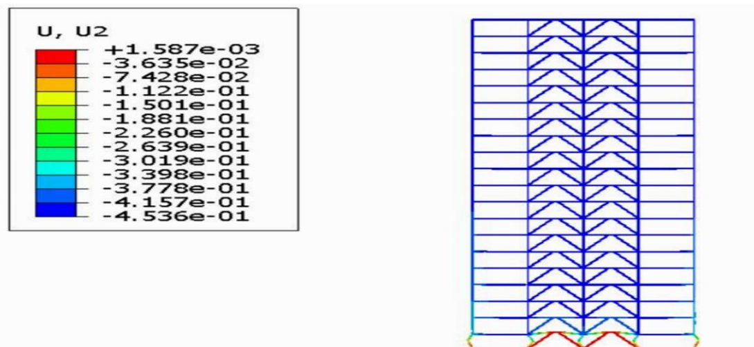
Figure 15: The highest displacement in thermal analysis in model number 13 (frame with diverging brace, 20-floor model, fire place in the middle of the first floor of the structure)
