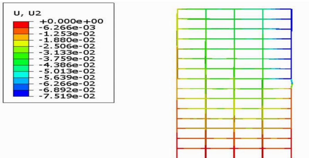
Figure 6: The highest displacement in thermal analysis in model number 4 (simple frame, 15-floor model, fire location next to the middle floor of the structure)
