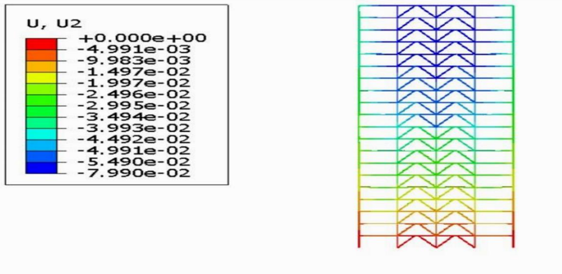
Figure17: The highest displacement in thermal analysis in model number 15 (frame with divergent brace, 20-floor model, fire place in the middle of the middle floor of the structure)
