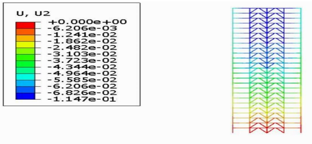
Figure 25: The highest displacement in thermal analysis in model number 23 (frame with divergent brace, 25-floor model, fire location in the middle of the middle floor of the structure)
