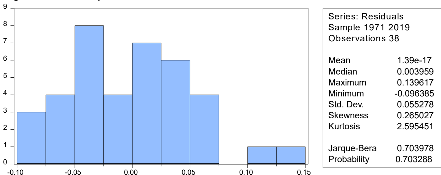
Figure 1: Normality test
