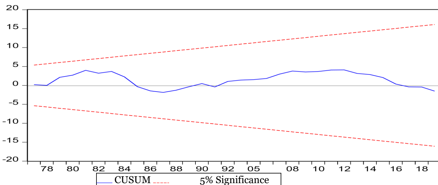
Figure 2: Cusum test (Cusum test)
