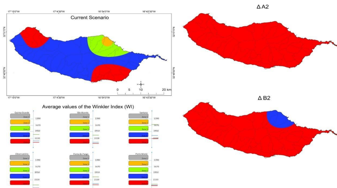
Figure 6. Interpolation of the Winkler Index (WI), for the current scenario and for the \Delta A2 and \Delta B2 scenarios proposed by Madeira Climate Strategy for 2070-2099 4. Conclusion
