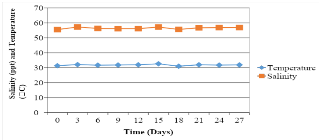
Figure 2: Temperature and salinity of brackish
