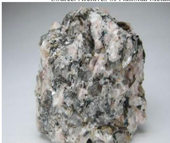
Plate iii: Pegmatite is a light-colored, extremely Coarse-grained intrusive igneous rock.
