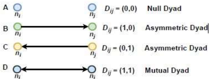
Figure 11. Dyadic isomorphism [55]
