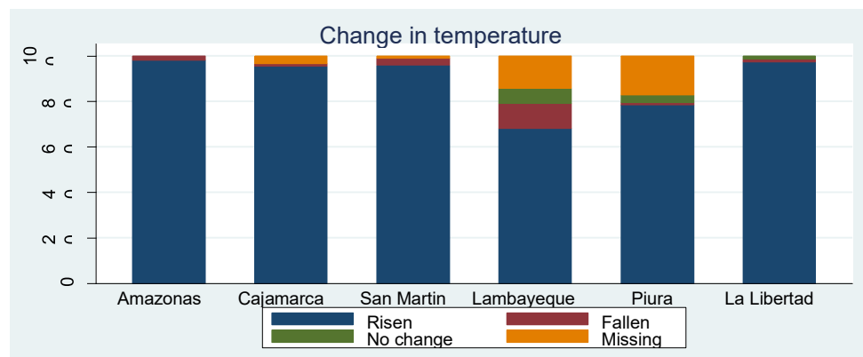
Figure 7. Hotter during hot seasons
