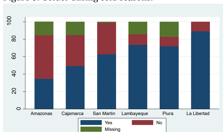
Figure 8. Colder during cold seasons.
