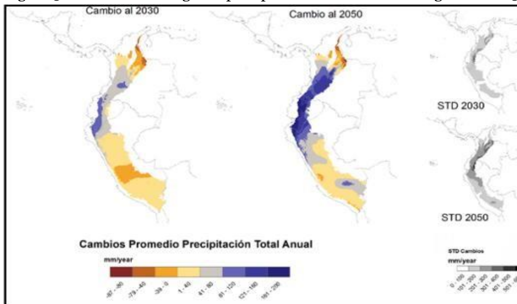
Figure 3. Forecasted changes in precipitation in the Andean region for 2030 and 2050.
