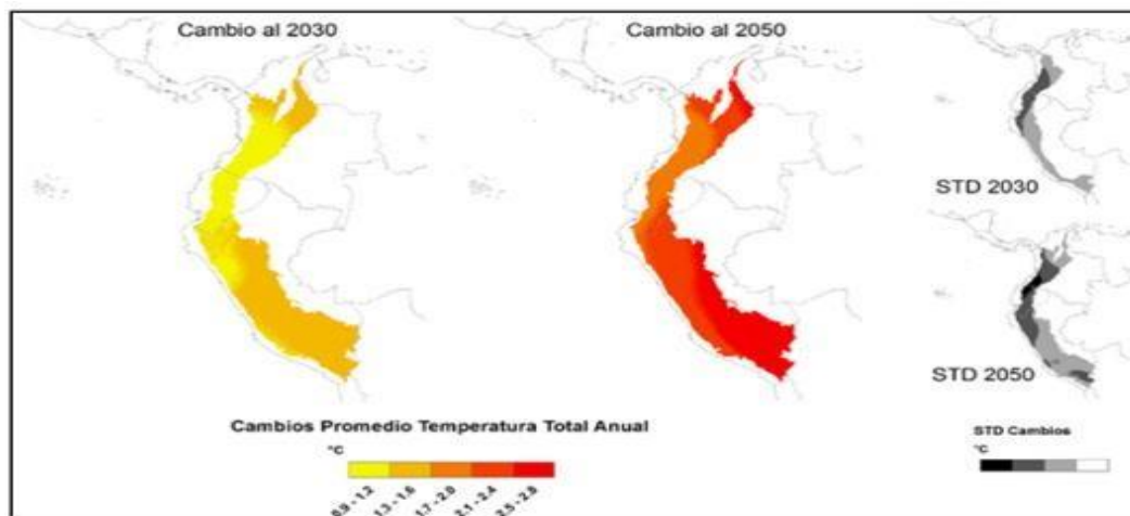
Figure 2. Forecasted changes in temperature in the Andean region for 2030 and 2050.
