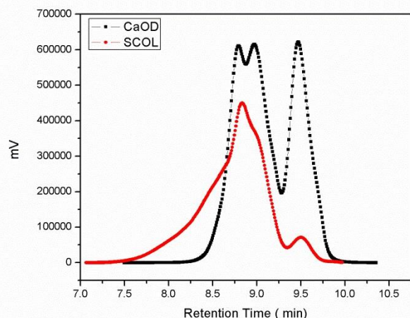
Figure 5. GPC Chromatogram of polyols.
