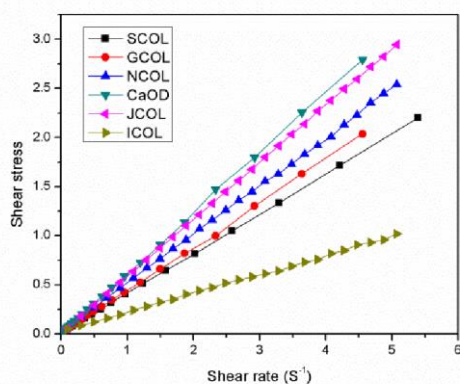
Fig. 6(a). Rheogram spectra of polyol and CaOD fatty diol
