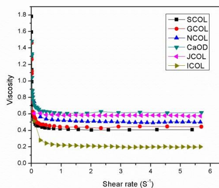
Fig. 6(a). Rheogram spectra of polyol and CaOD fatty diol
