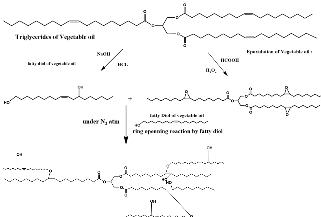
Schematic Representation of epoxies and polyols from vegetable oils.
