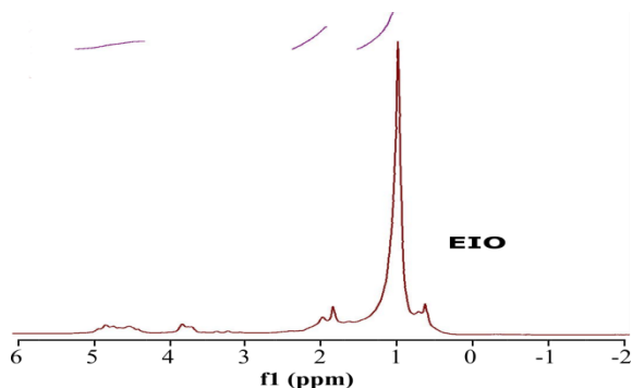
Figure. 2(a) to 2(e) ^1\text{H} NMR spectra of epoxidised vegetable oils.
