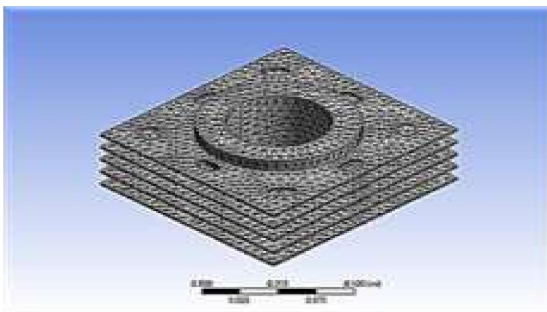
Figure 6. Mesh model of rectangular fin.
