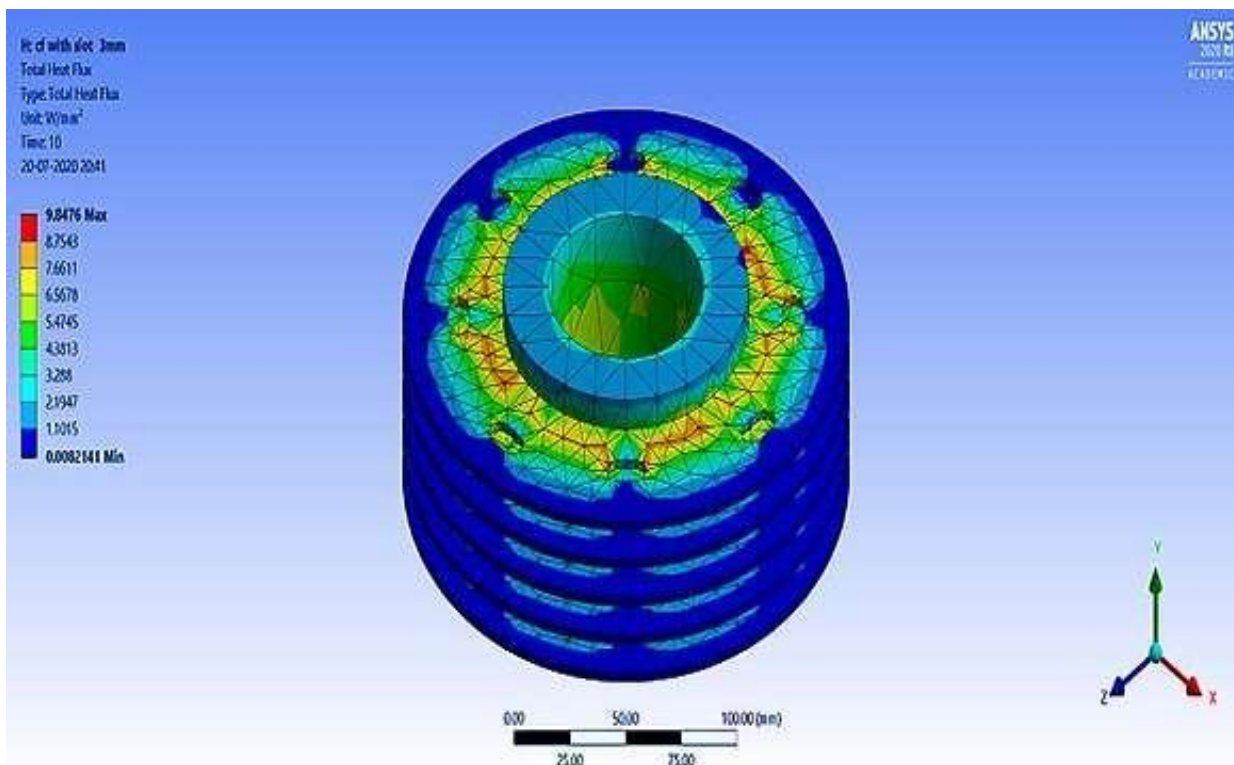
Figure 24. Total heat transfer per unit area in circular fin 3 mm without slot.
