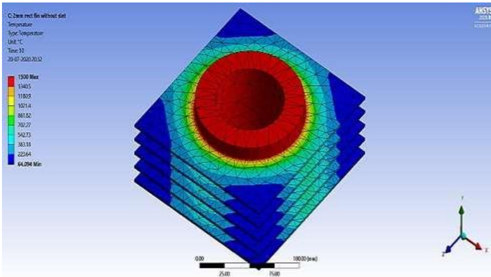
Figure 10. Temperature distribution in rectangular fin 2 mm thickness without slot.
