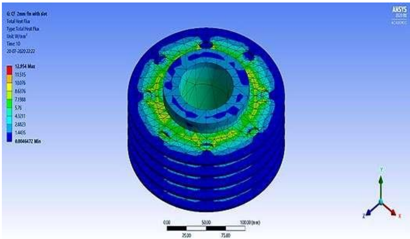
Figure 22. Total heat transfer per unit area in circular fin 2 mm without slot.
