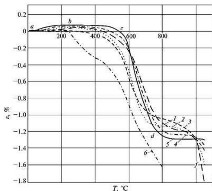
Figure 4. Dependence of the relative thermal deformation of fiberglass
