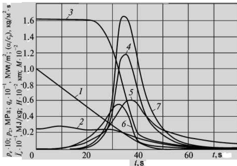
Figure 1. Dependence of parameters of gaseous dynamic flow acting on a side surface of a re-entry spacecraft vs. descent time t from the Earth orbit ( H - 1; M - 3; I_e - 3; p_e - 4; \alpha/c_p - 5; q_e - 6; p_\Sigma - 7) [1].
