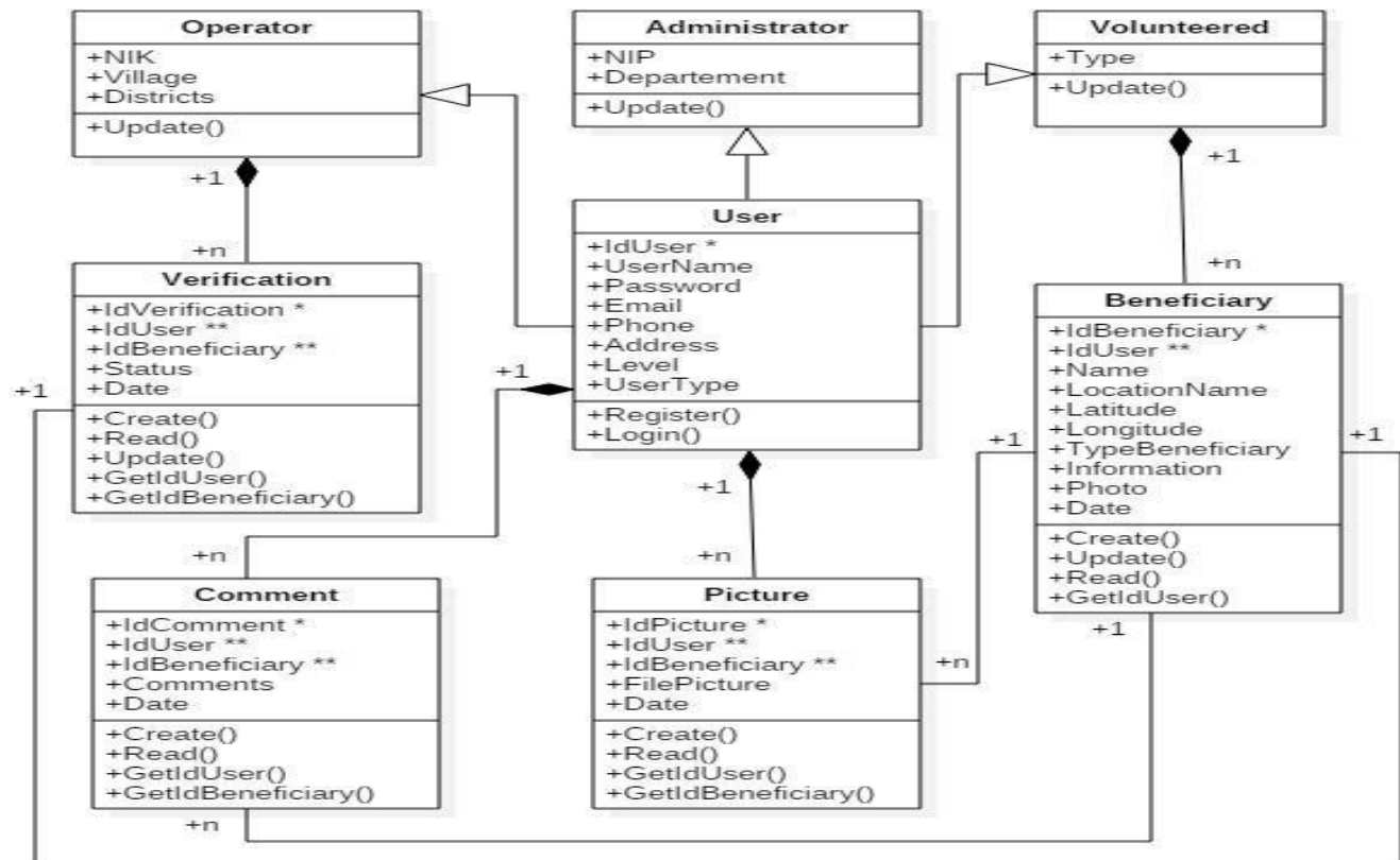
Fig 7. Class diagrams of Infrastructure Model VGI Social Assistance Program
