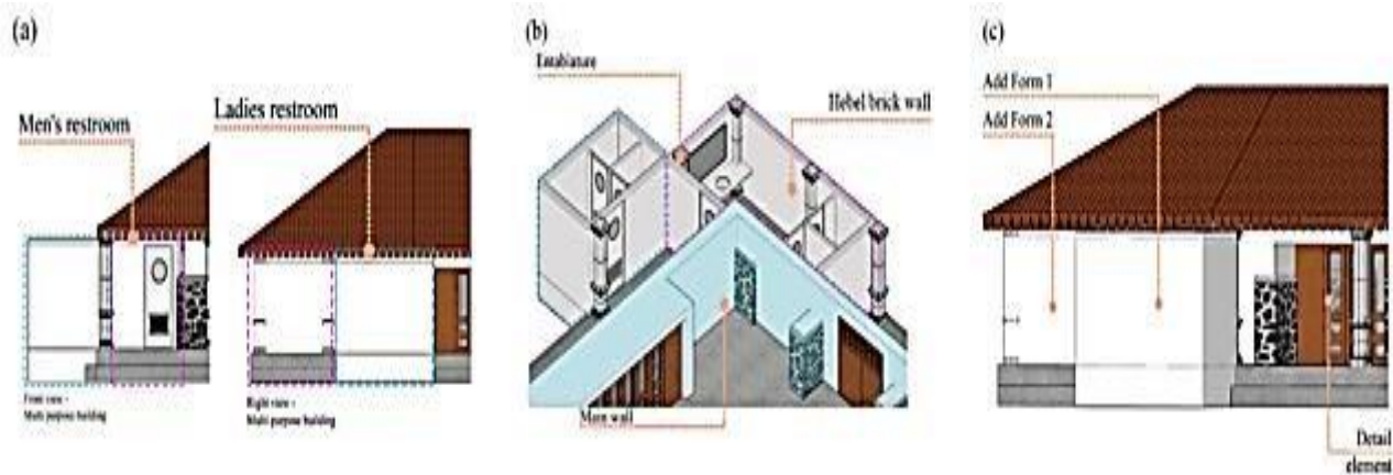
Fig 3. Analysis of conservation activities that occur in the Multipurpose building. (a) Adding a new shape to the back area of the Multipurpose building that functions as a men's and women's toilet, (b) Identification the effect of the wall area or the shape of the new building on the structure of the Multipurpose building, (c) Identification of additional forms and their effects on the detail elements of the facade. Source: Mahendra, 2018 (reprocessed)
