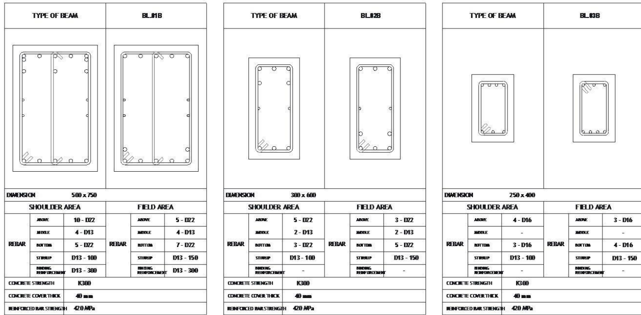
BEAM REINFORCED BAR DETAIL SKALA 1:10
