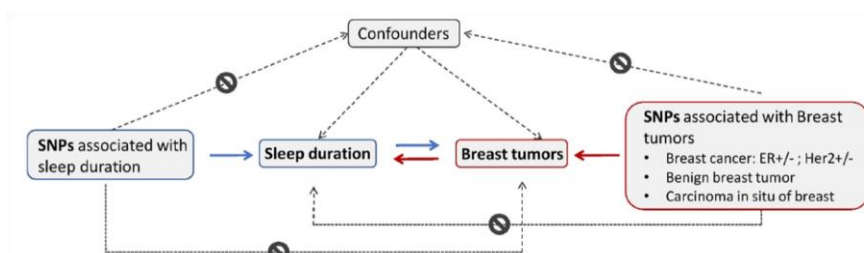
Figure 1. Workflow of this bidirectional Mendelian Randomization (MR) study.
